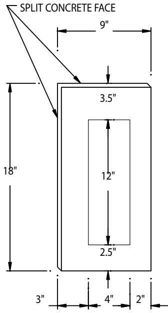
90° CORNER UNIT
