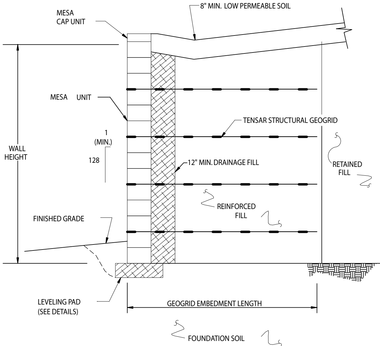
TYPICAL CROSS-SECTION
